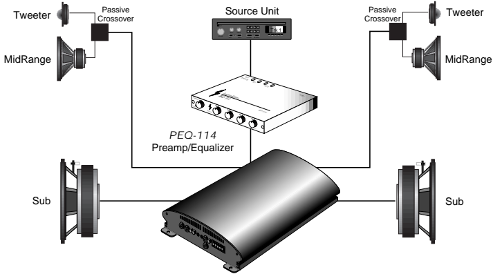
POWERCLASS™ Amplifier PC4200, PC4400 or PC4800 Front High Pass 100Hz Rear Low Pass 100Hz
